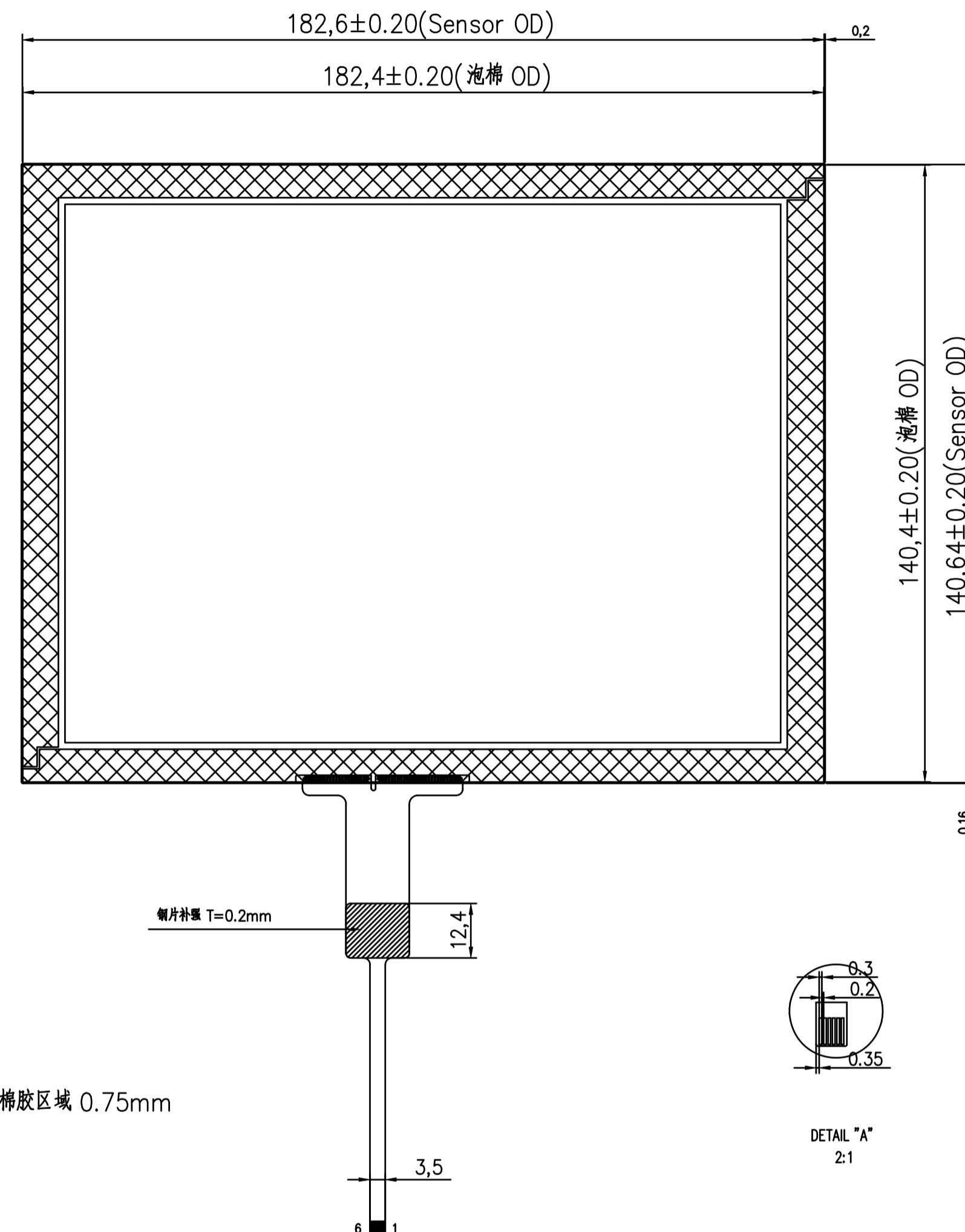
Back view
