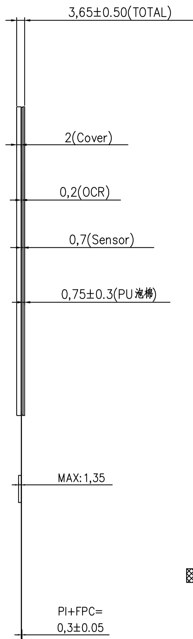
Side view
